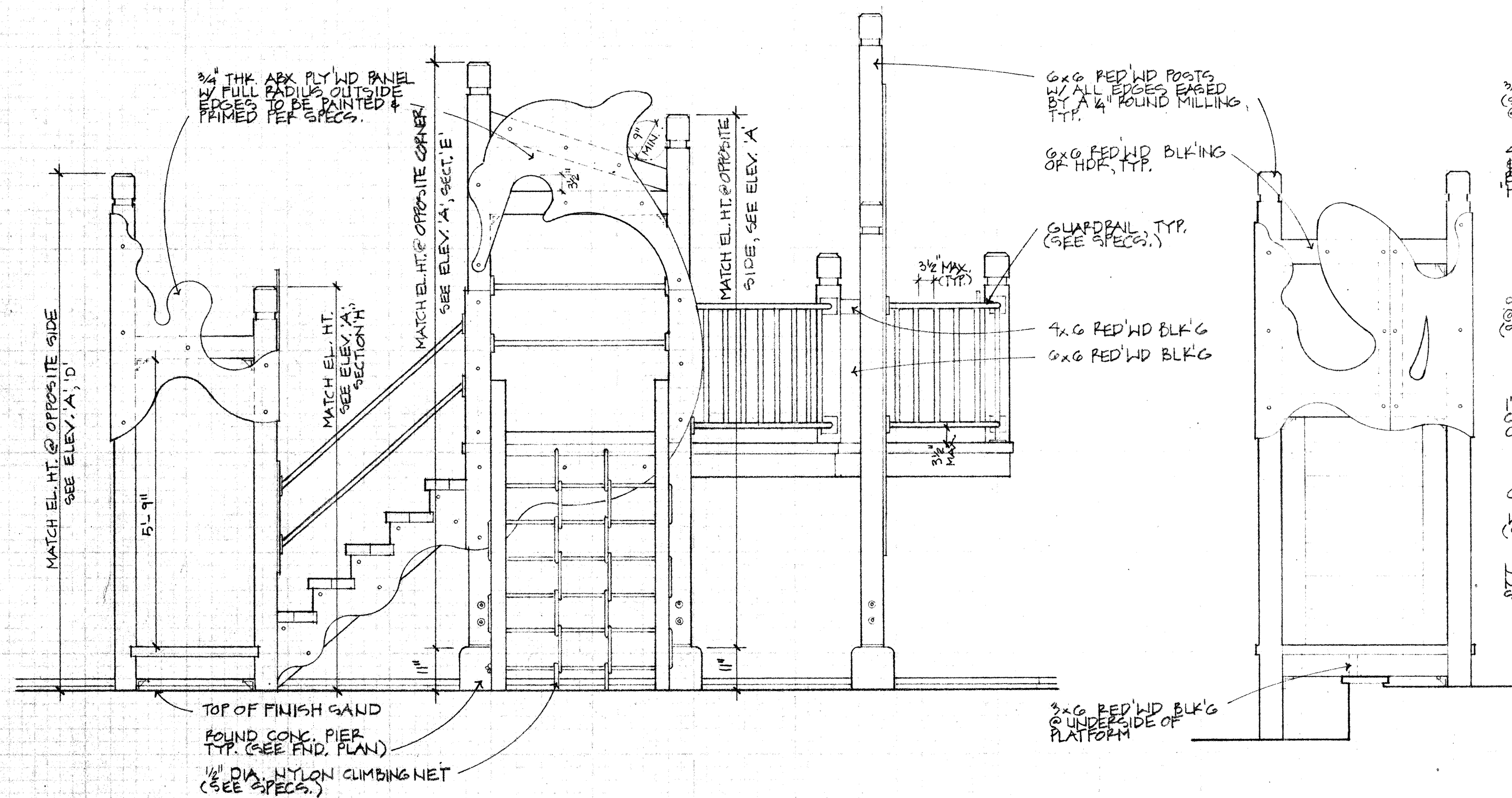
Elevation C
