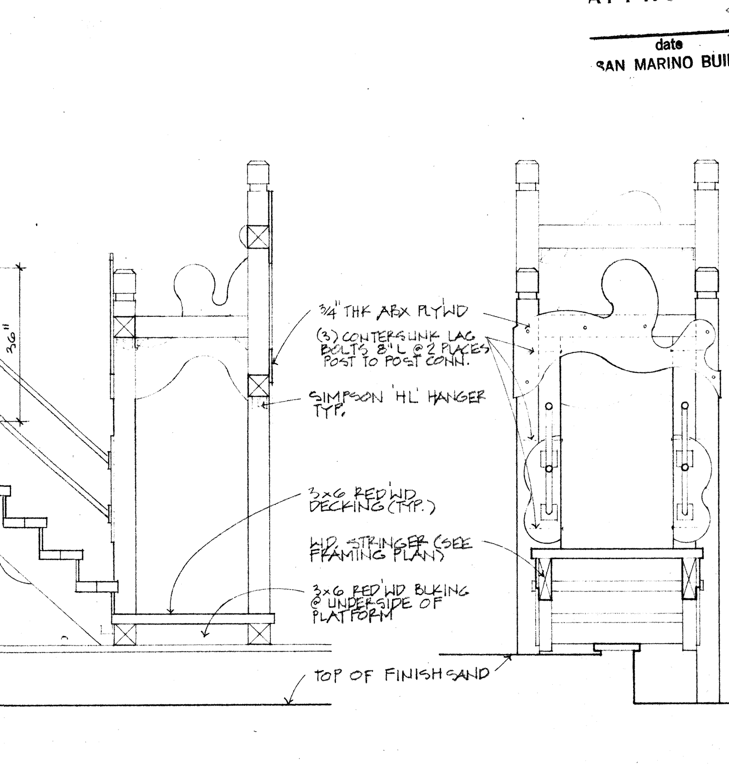
Section G
